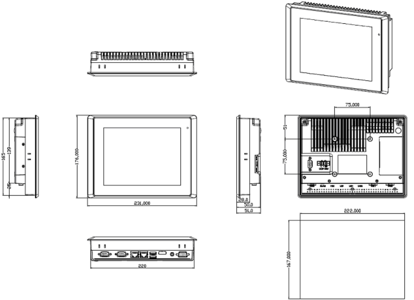
Mounting Hole Size
