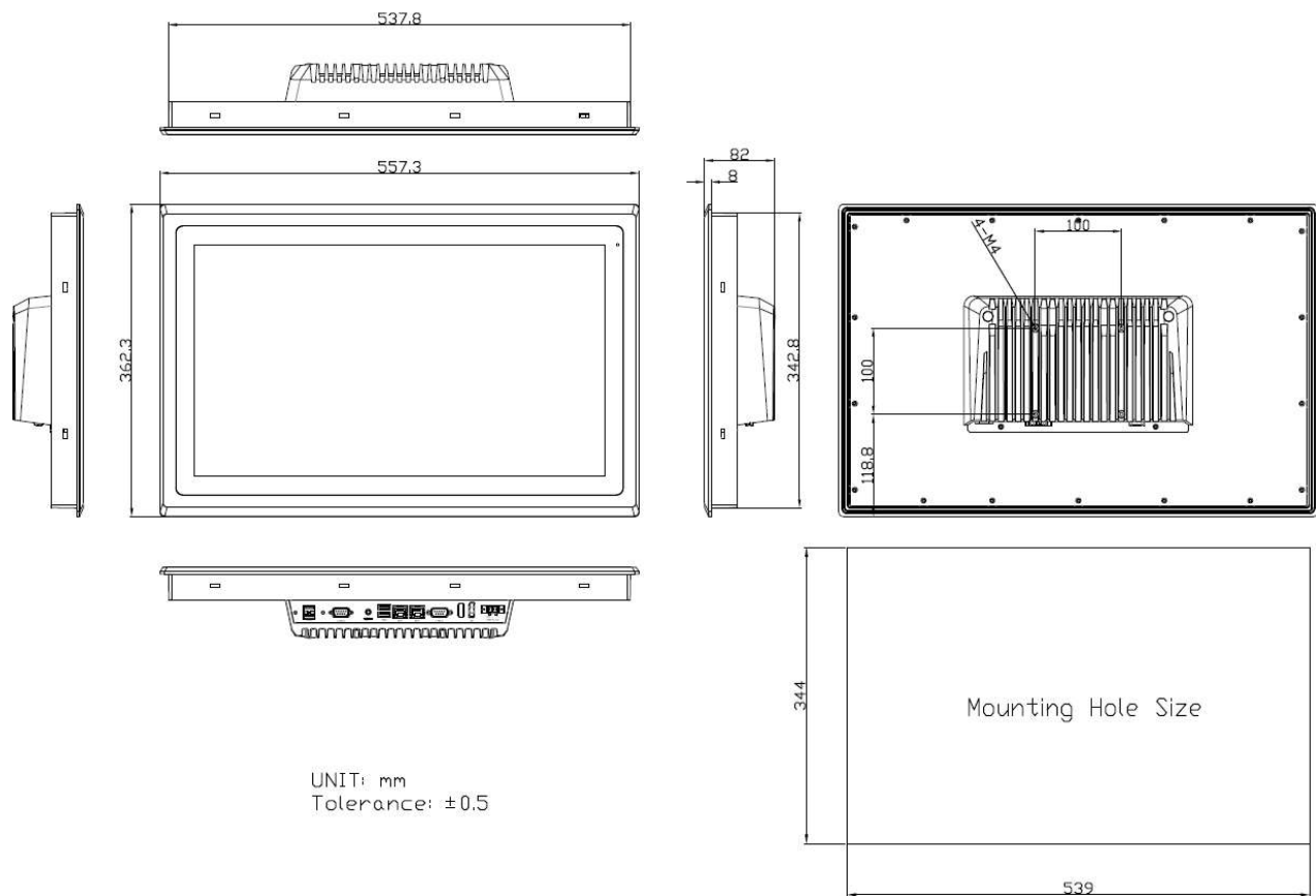
Figure 11 Dimensions of NP-621-S
