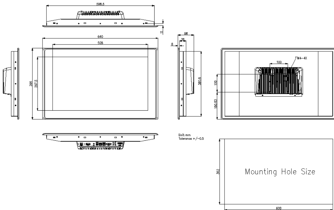
Figure 12 Dimensions of NP-624-S
