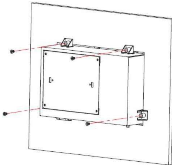
Figure 17 NP-6XX-S PANEL Mounting
