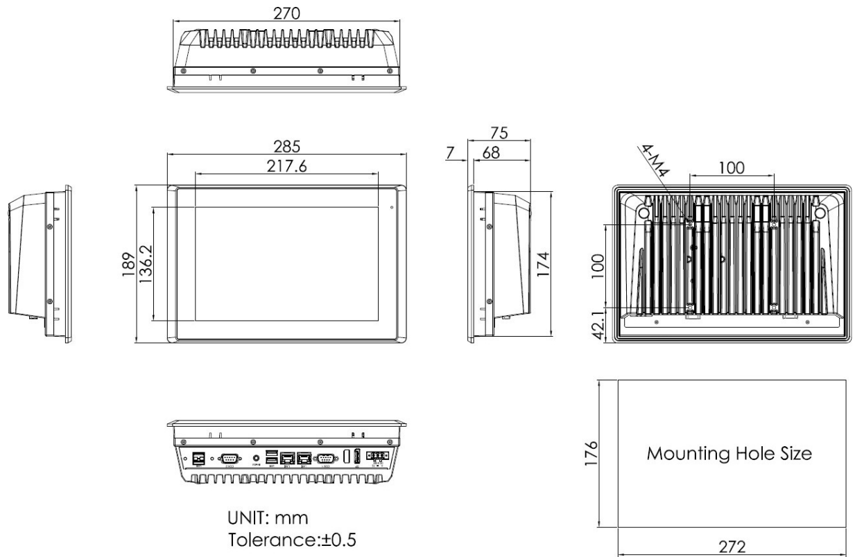
Figure 3 Dimensions of NP-610-S
