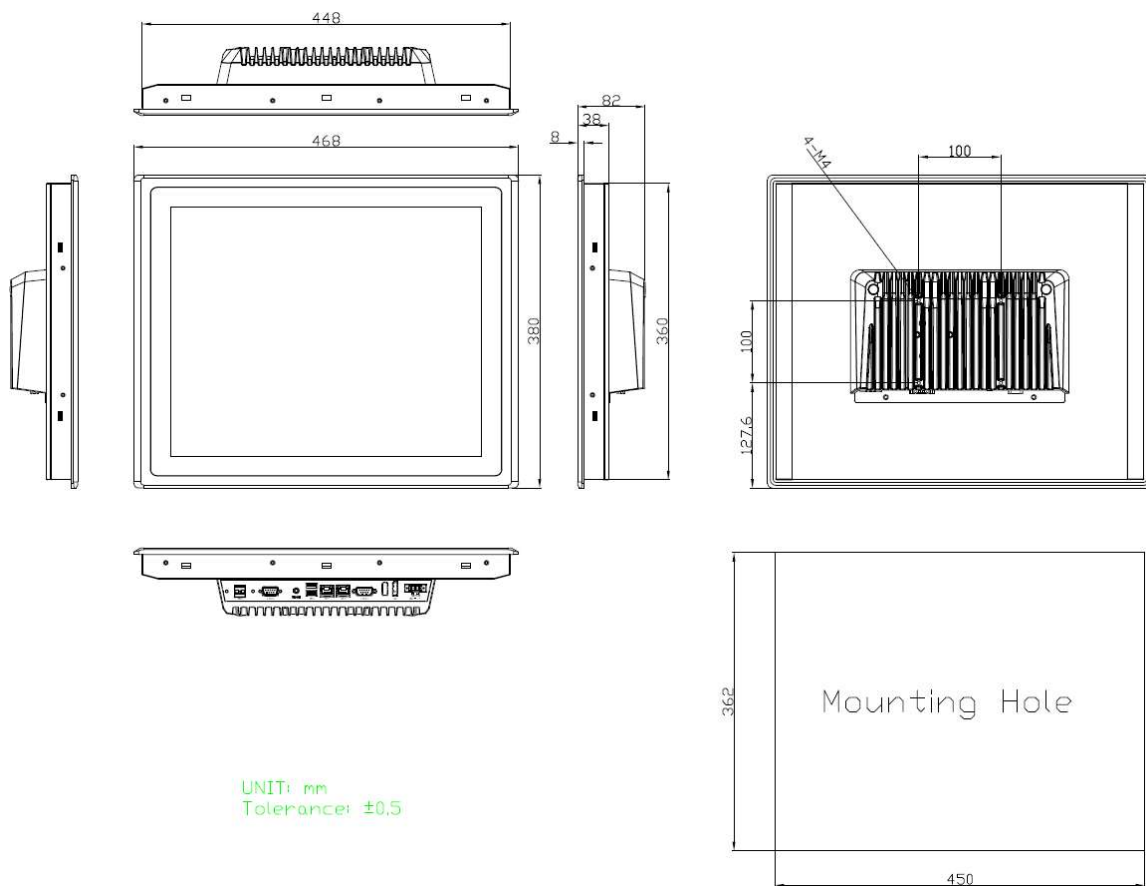
Figure 10 Dimensions of NP-619-S
