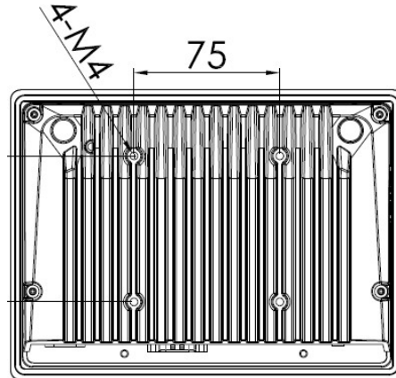
Figure 15 NP-607-S/608-S VESA Mounting
