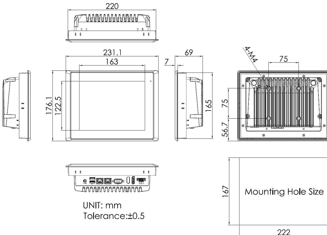
Figure 2 Dimensions of NP-608-S
