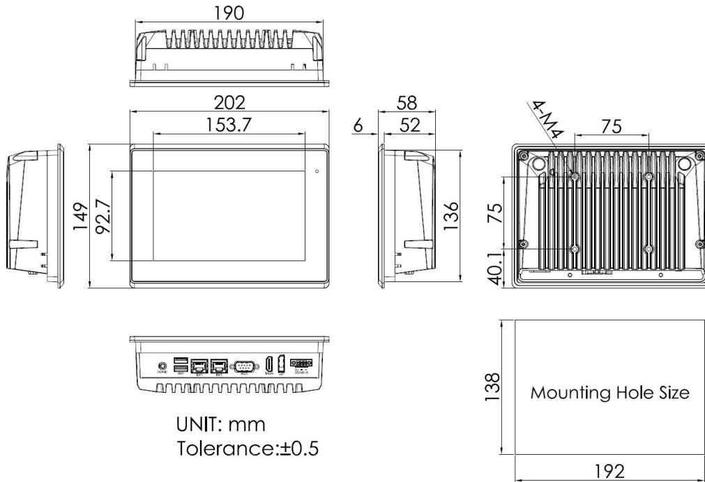
Figure 1 Dimensions of NP-607-S
