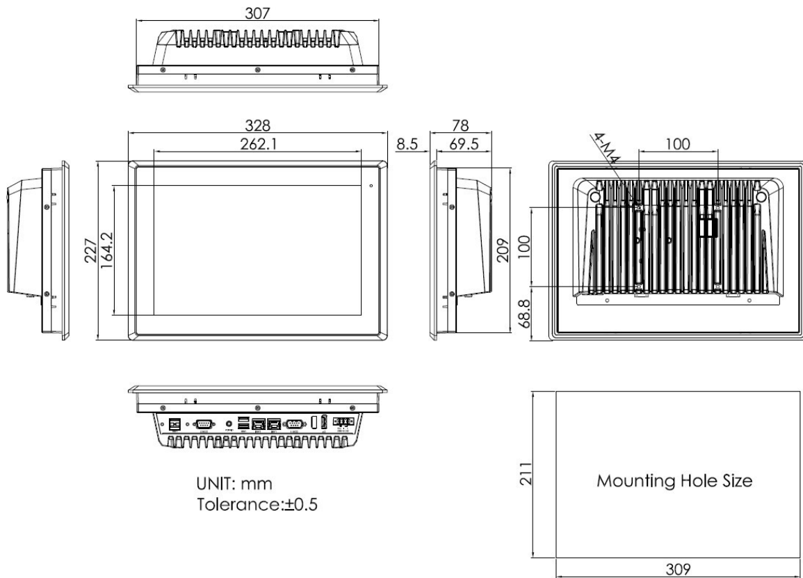
Figure 5 Dimensions of NP-612
