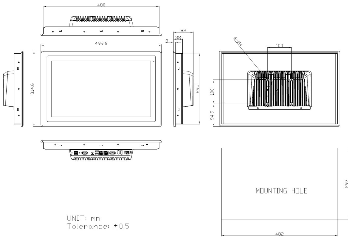
Figure 9 Dimensions of NP-618-S/R(H)
