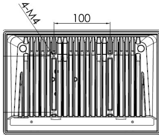
Figure 16 NP-610-S/612-S/612W-S/615-S/616-S/617-S/618-S/619-S/621-S/624-S VESA Mounting
